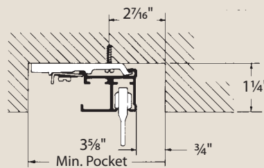
No. 94130 Bracket for recess mounting
